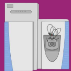
Mass Spectrometry
